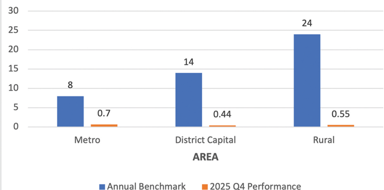
CAIDI (Hours/Customer)
