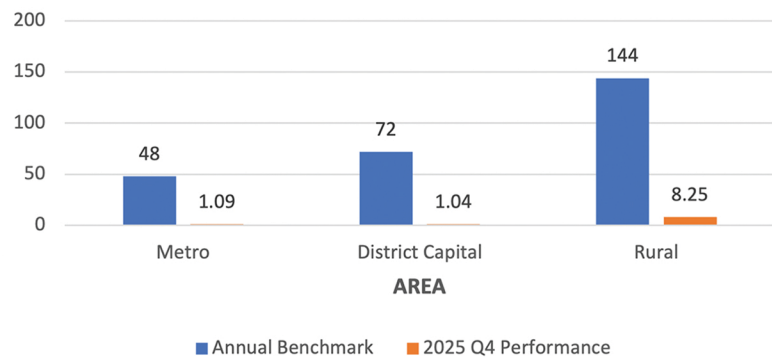
SAIDI (Hours/Customer)
