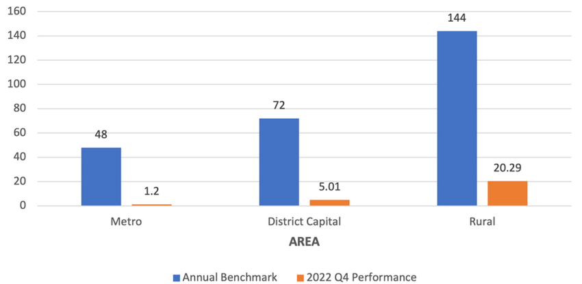
SAIDI (Hours/Customer)
