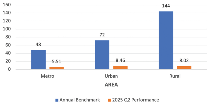
SAIDI (Hours/Customer)
