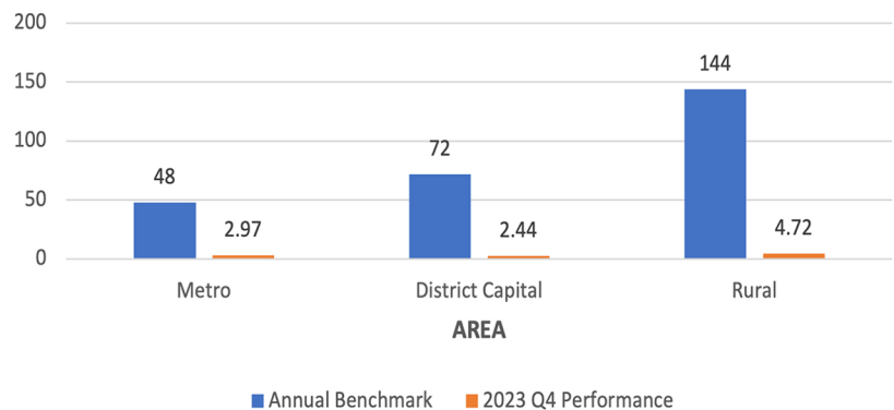
SAIDI (Hours/Customer)
