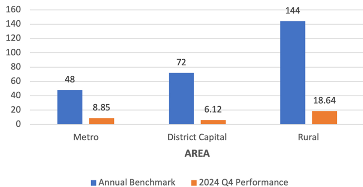
SAIDI (Hours/Customer)
