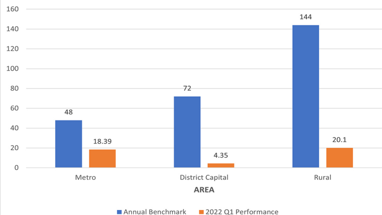
SAIDI (Hours/Customer)
